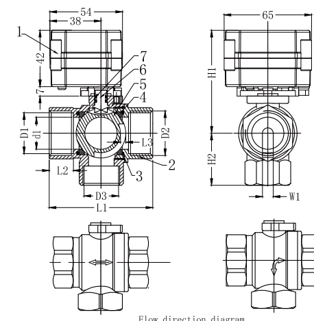
Flow direction diagram
